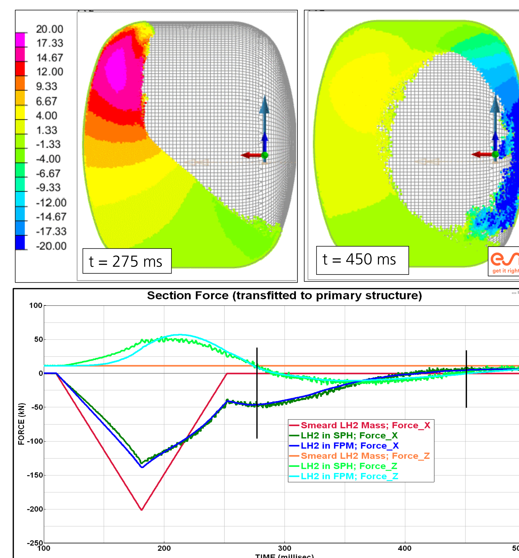
Exemplary results of fuel sloshing assessment using a 2-way coupled CFD / CSM method (FPM):
