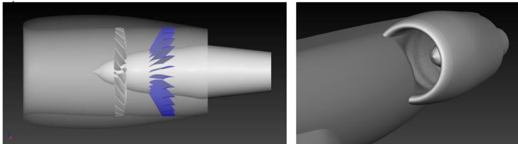
Figure 3: SDT low-noise fan stage with modified nacelle (left) and nacelle integration on NOVA fuselage with an s-duct (right) (© TU Delft, 2018)
